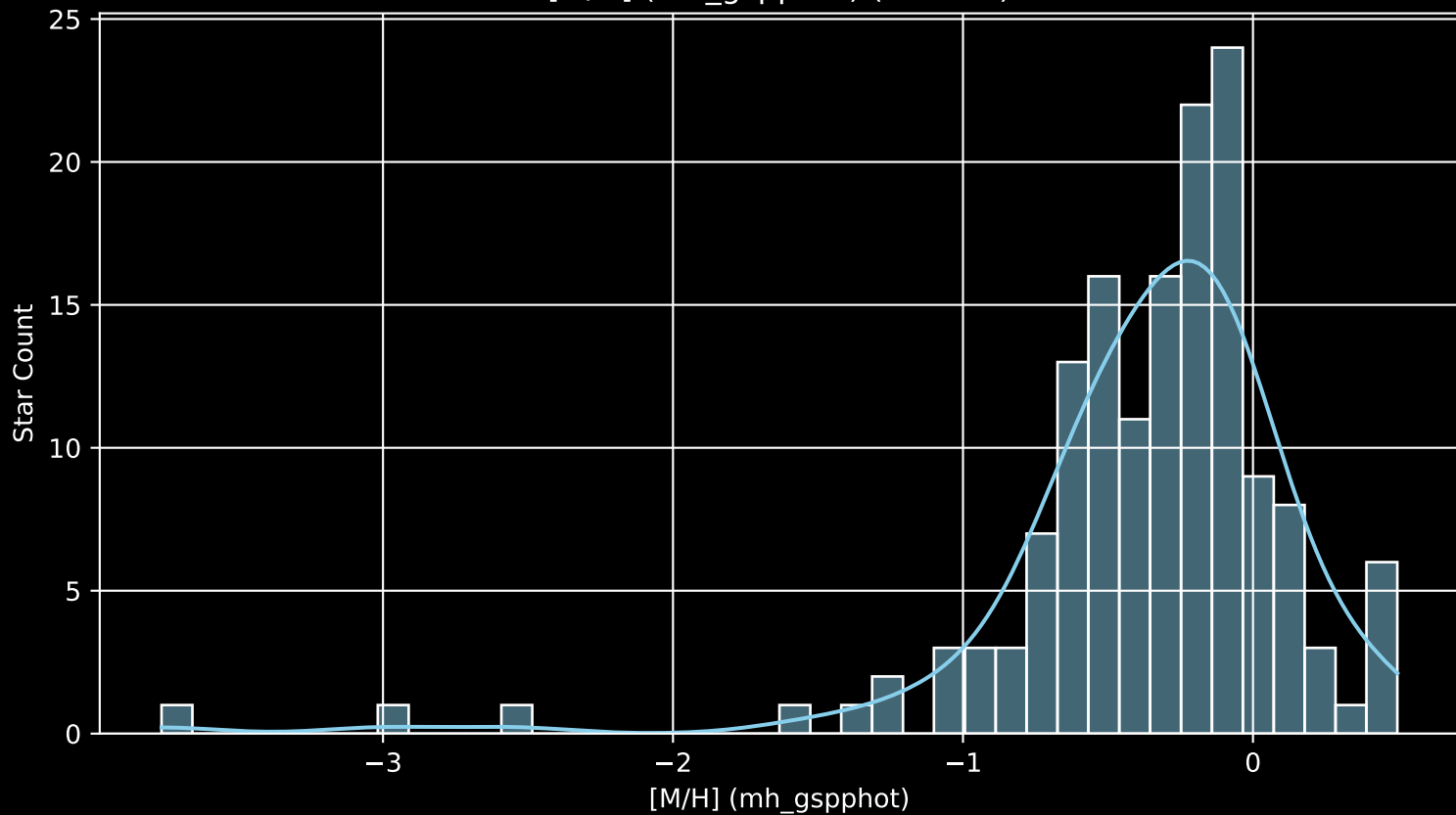
APOGEE DR17 Field: [355+22-O [M/H] (mh_gspphot) (n= 152)
