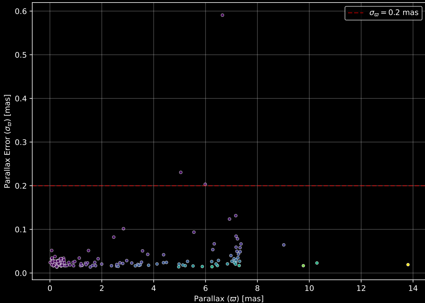
APOGEE DR17 Field: [355+22-O] Parallax Quality (n= 153)
