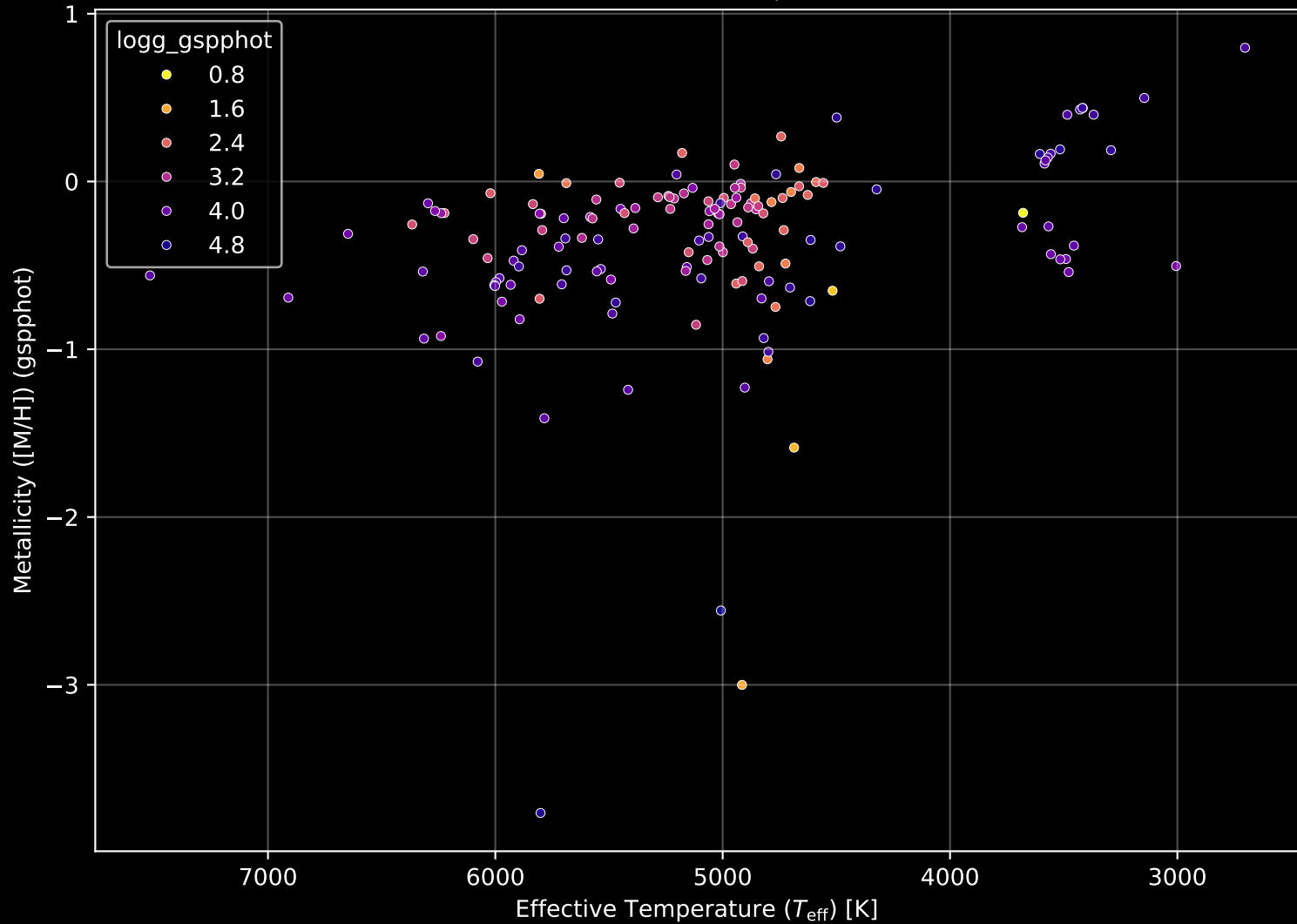
APOGEE DR17 Field: [355+22-O] Stellar Population Parameters (n= 153)
