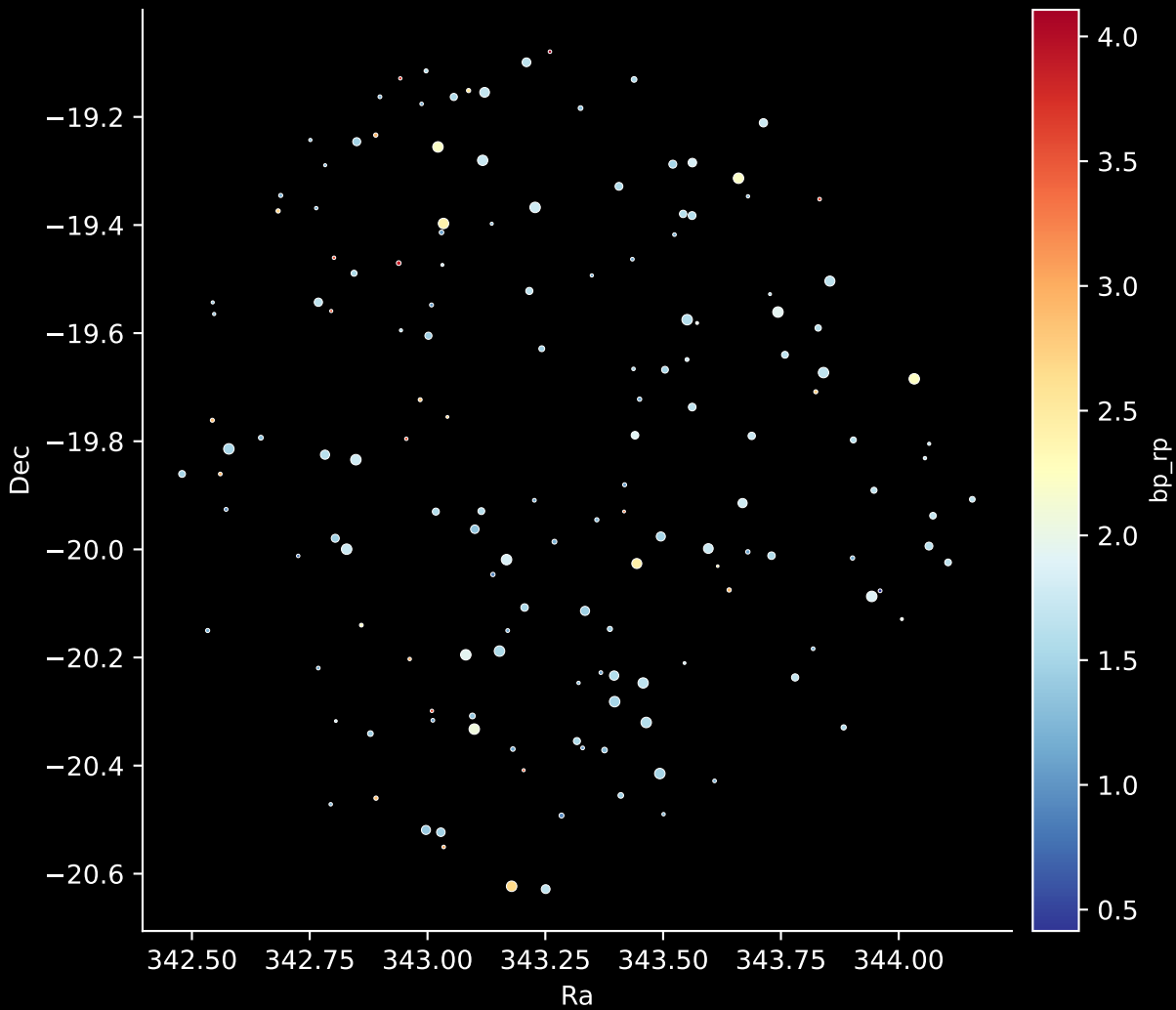
APOGEE DR17 Field: [355+22-O] Stars: 153
