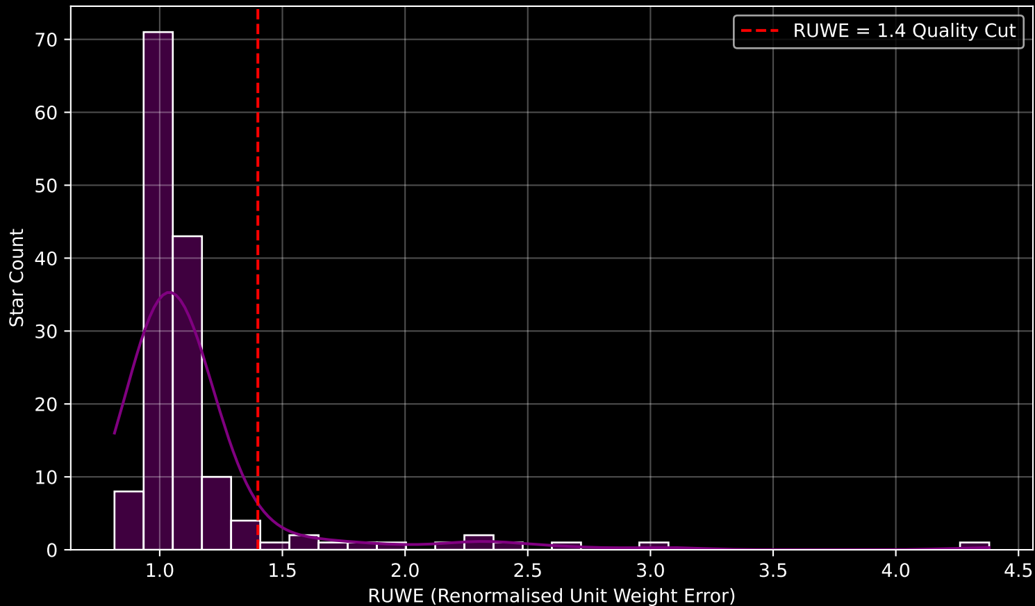
GAPOGEE DR17 Field [355+22-O] RUWE Distribution (n= 149)
