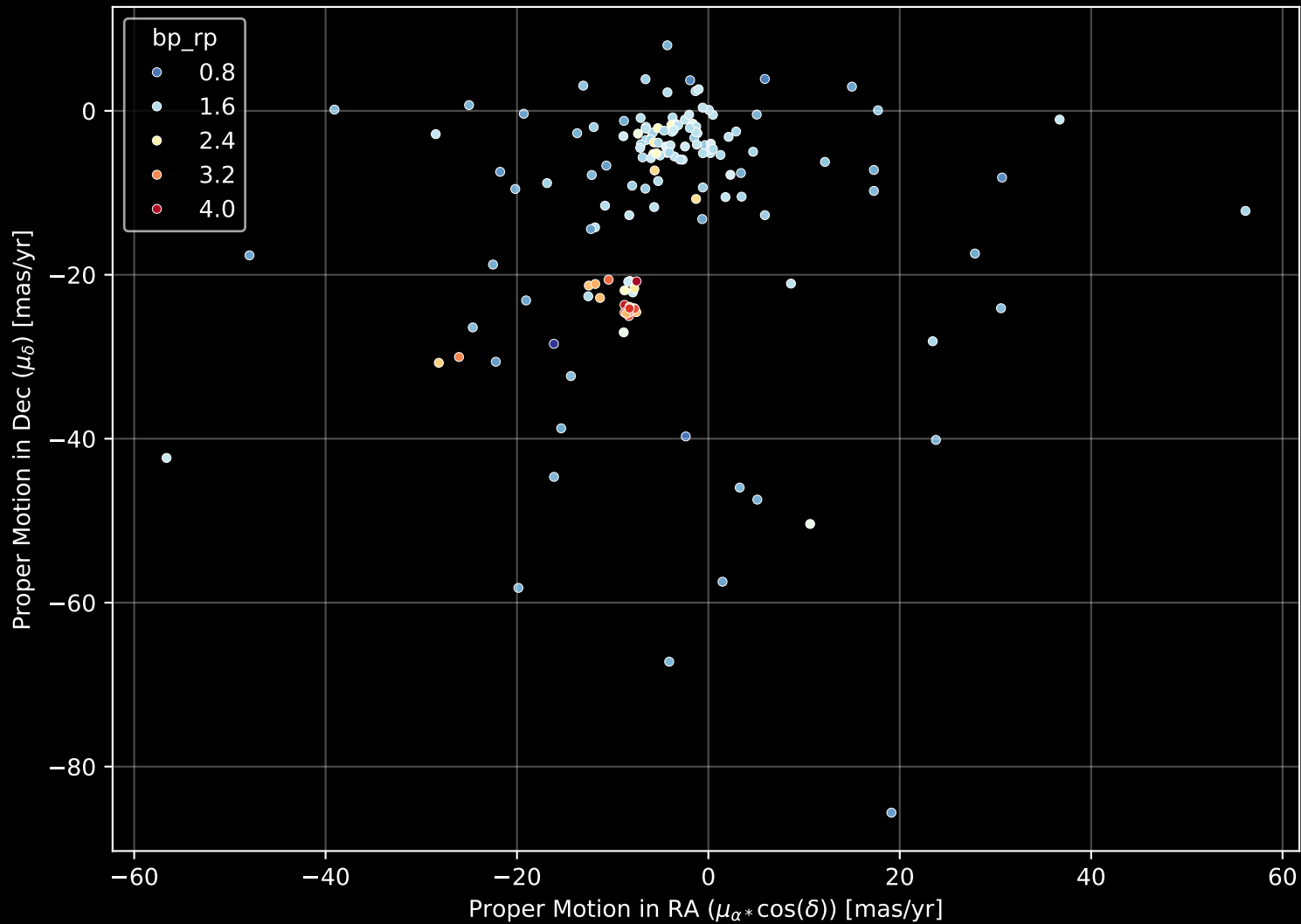
APOGEE DR17 Field: [355+22-O] Proper Motion Diagram (n= 153)
