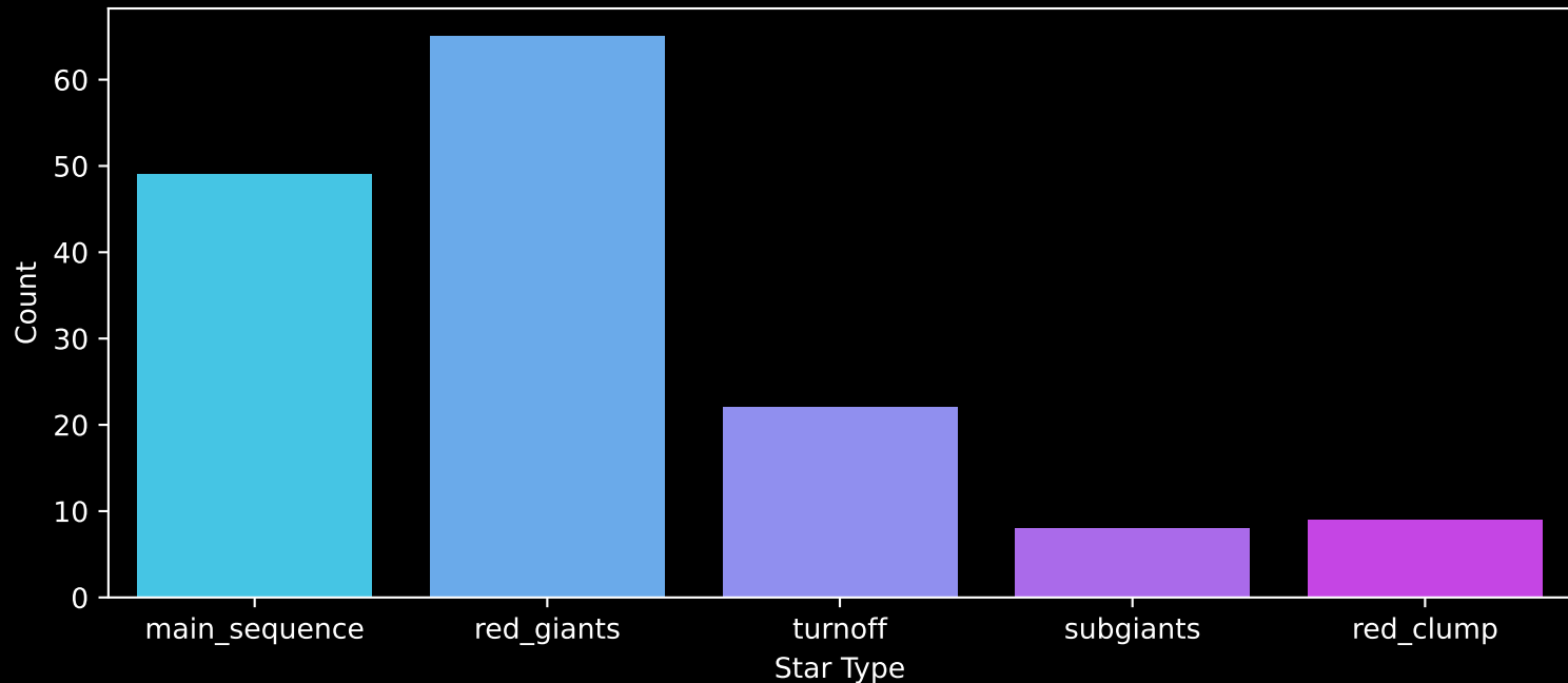
APOGEE DR17 Field: [355+22-O] Count plot of Star Type
